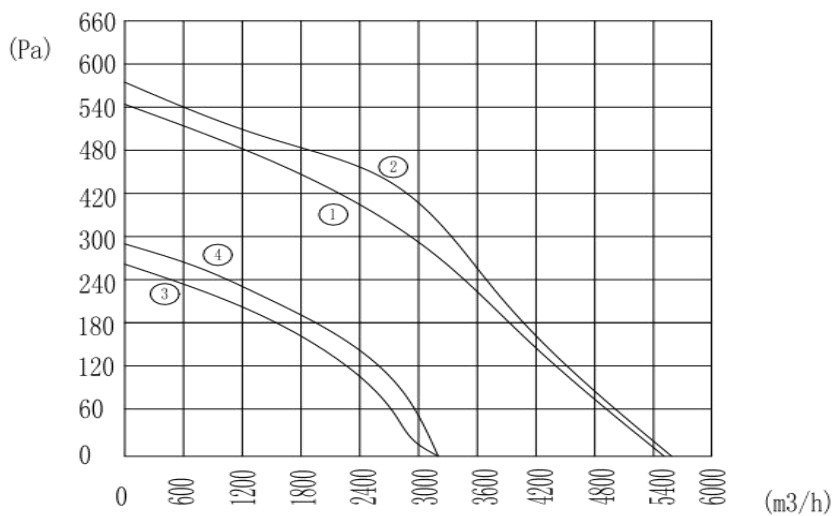
流量曲线/Airflow curves:
