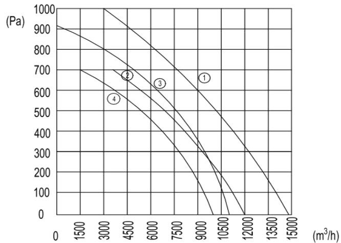
流量曲线/Airflow curves:
