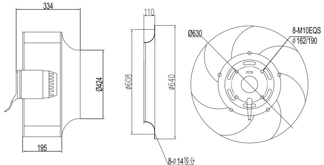
尺寸图/Dimensions:
