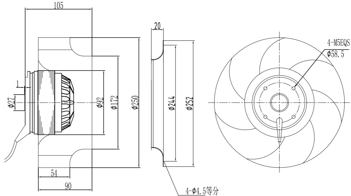
尺寸图/Dimensions:
