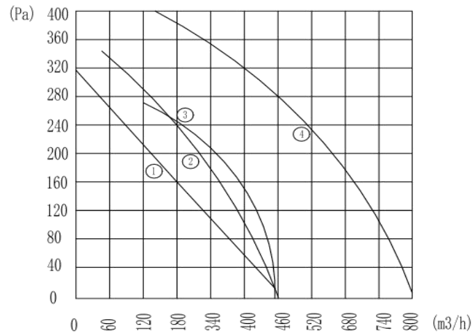
流量曲线/Airflow curves:
