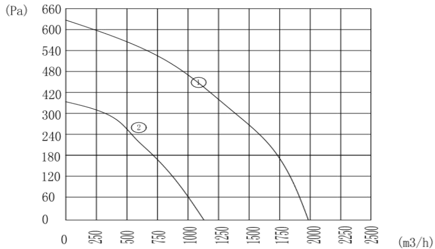
流量曲线/Airflow curves:
