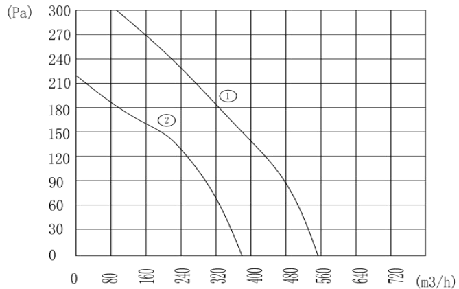
流量曲线/Airflow curves:
