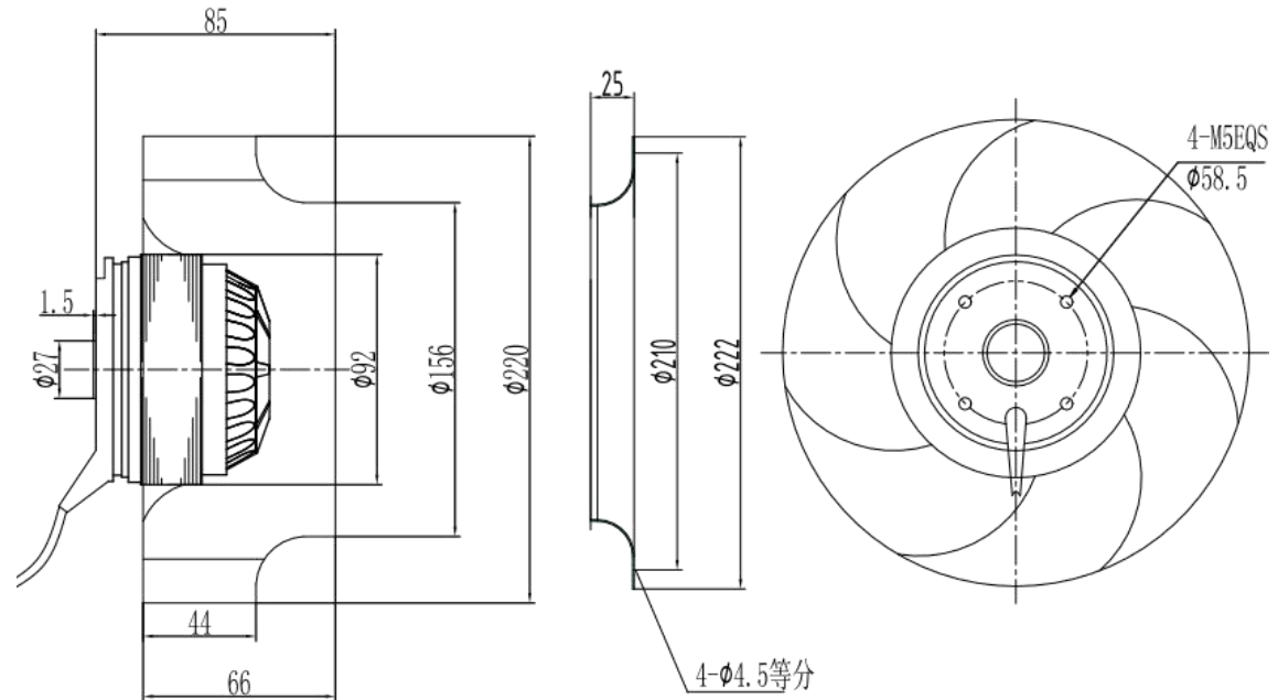
尺寸图/Dimensions:
