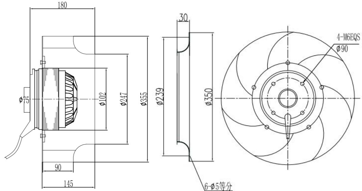
尺寸图/Dimensions:
