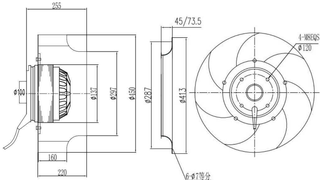
尺寸图/Dimensions:
