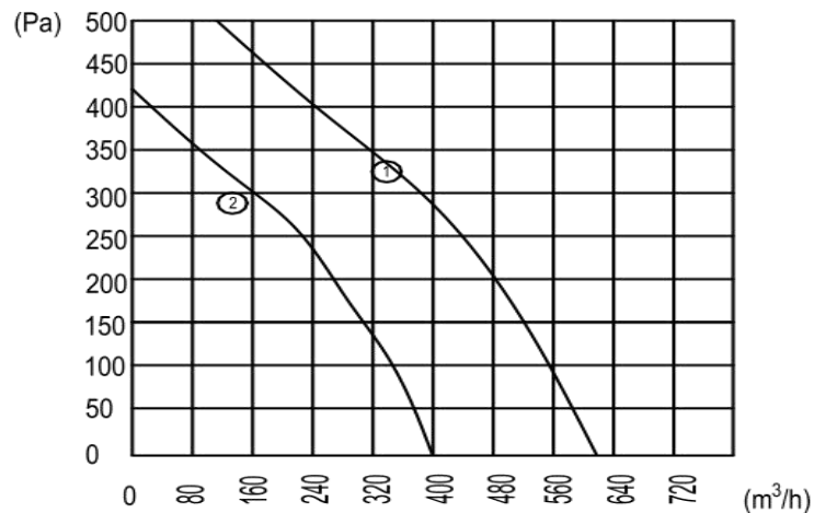
流量曲线/Airflow curves:
