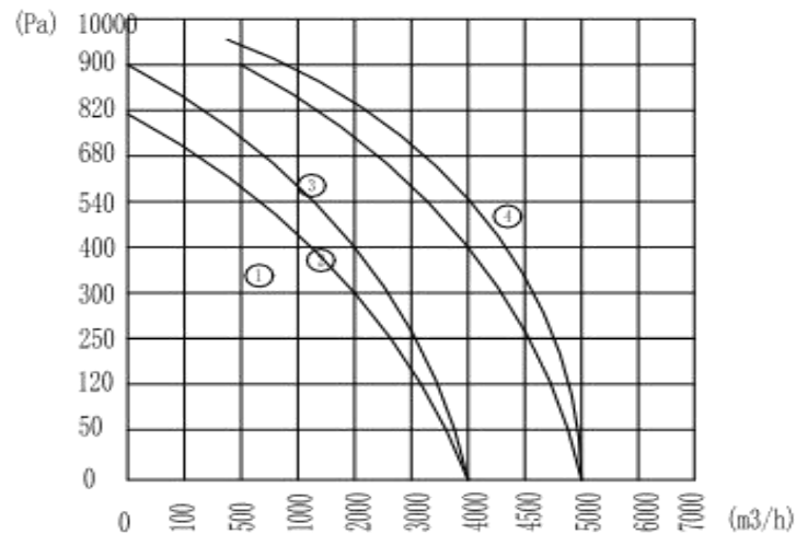
流量曲线/Airflow curves:
