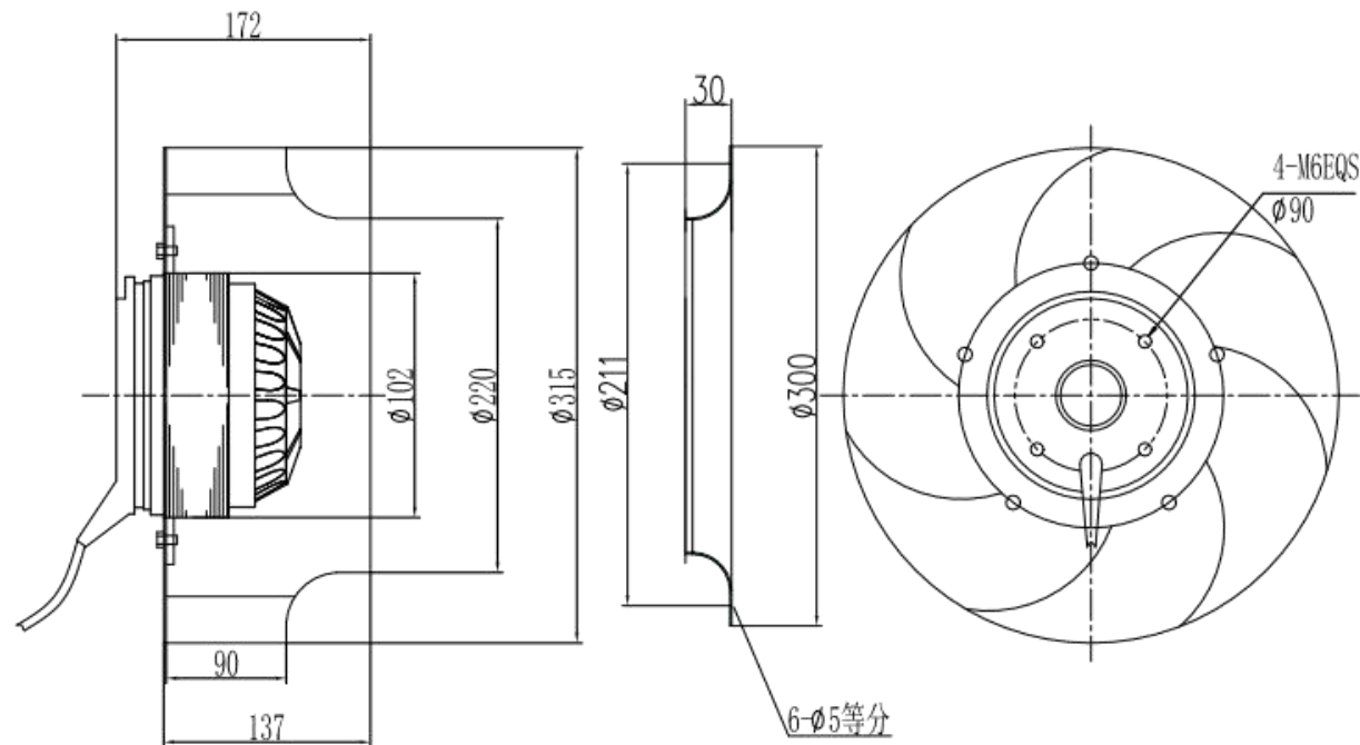
尺寸图/Dimensions:
