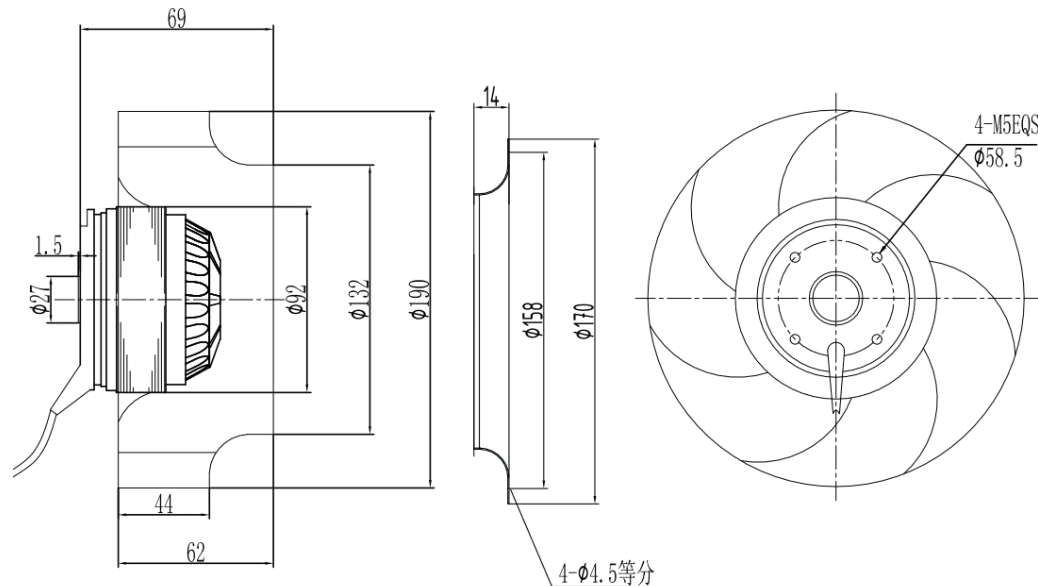
尺寸图/Dimensions:
