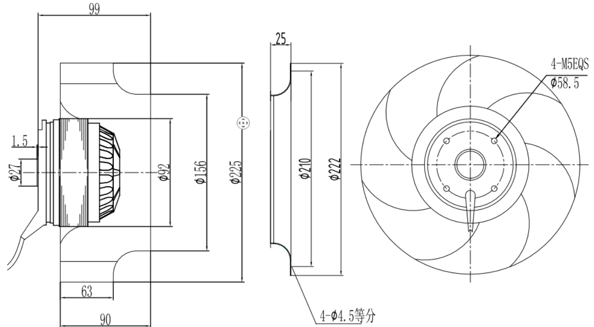
尺寸图/Dimensions:
