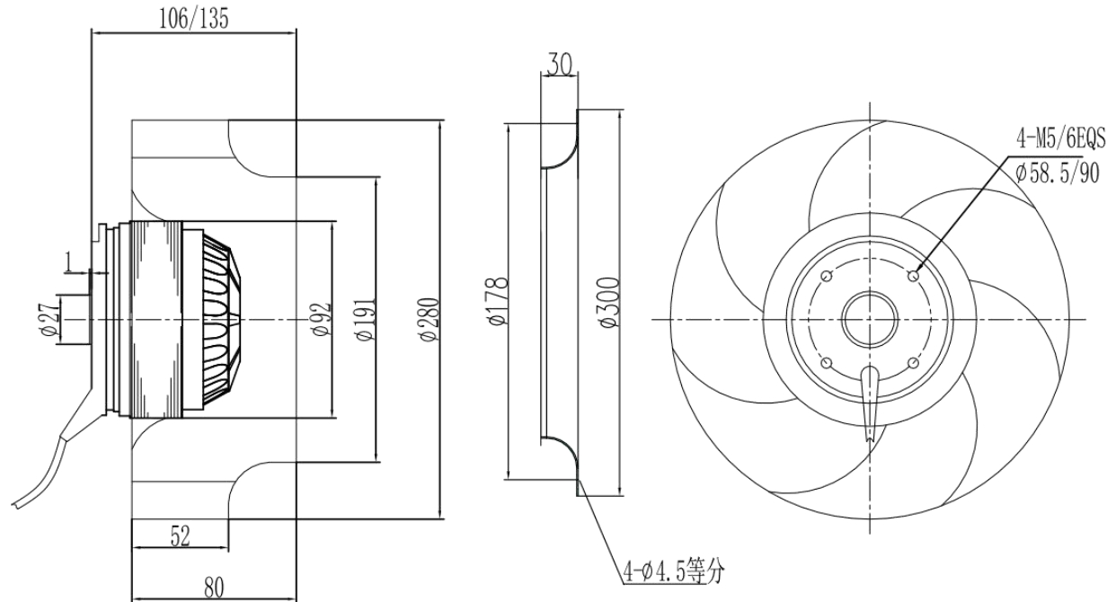
尺寸图/Dimensions:
