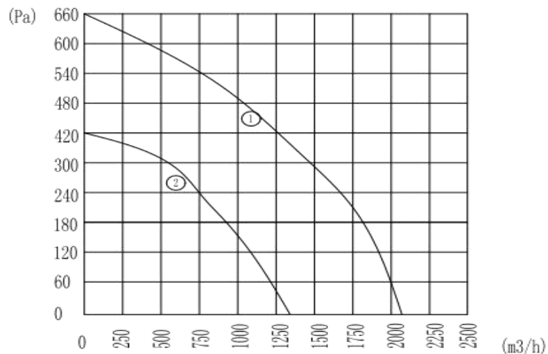
流量曲线/Airflow curves:
