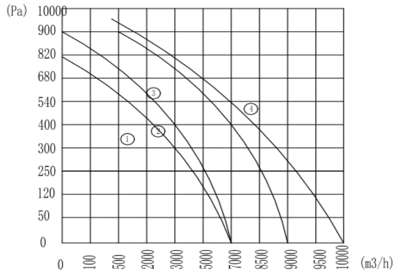
流量曲线/Airflow curves:
