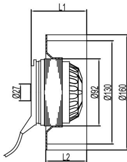
尺寸图/Dimensions:
