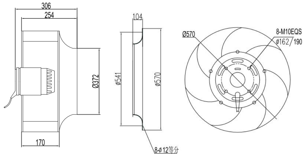
尺寸图/Dimensions:
