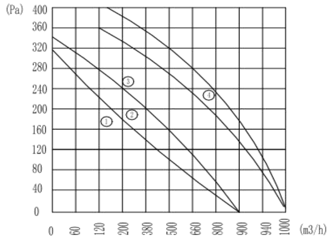
流量曲线/Airflow curves:
