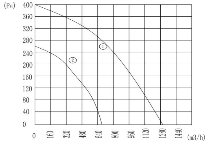
流量曲线/Airflow curves:
