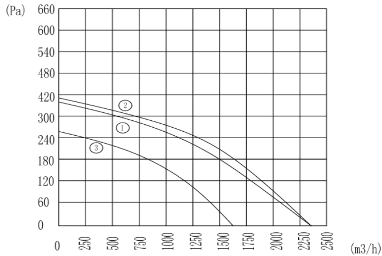
流量曲线/Airflow curves:
