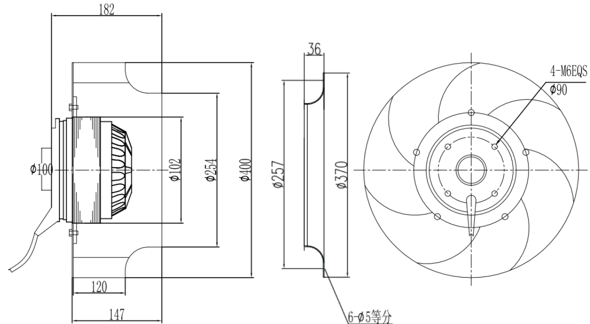
尺寸图/Dimensions:
