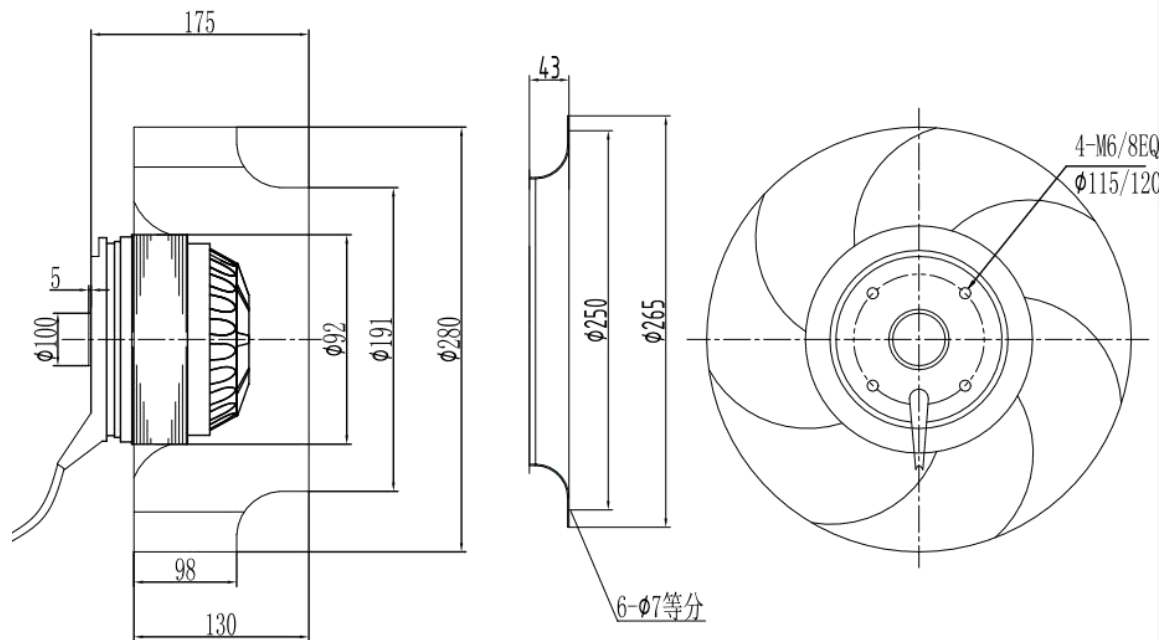
尺寸图/Dimensions:
